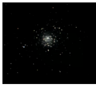
M5, three 5 second exposures stacked using the SkyRaider DS16CTEC on a 10" VRC.
