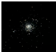
M5, four 5 second exposures stacked using the SkyRaider DS16CTEC on a 10" VRC.
